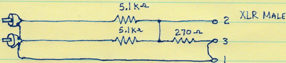
RCA Stereo to XLR Mic IN 2 EACH
